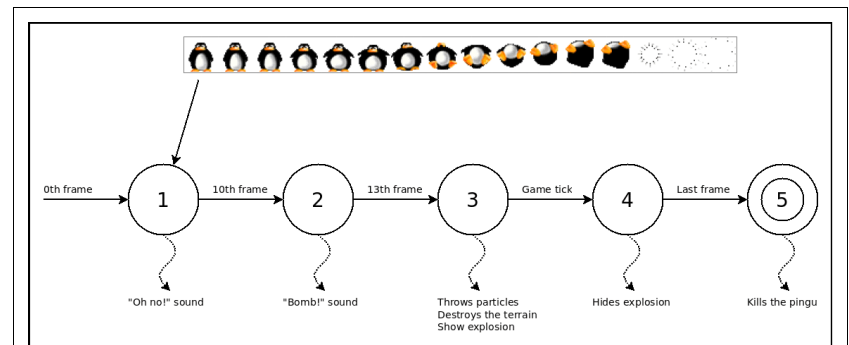
Figure 6: State machine for the Bomber animation
